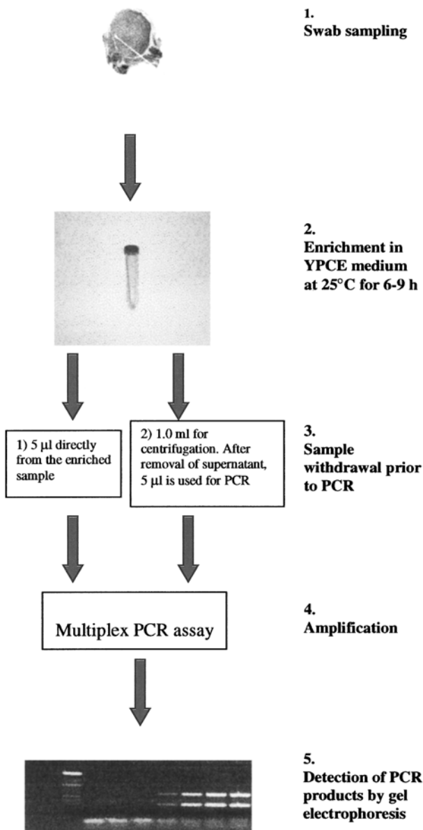
Fig. 2. An overview of the protocol ( see Subheadings 3.1.–3.4. ) illustrating the different steps. The protocol starts with swab sampling, followed by enrichment in YPCE medium at 25°C. After 6–9 h enrichment PCR samples are withdrawn; one sample is withdrawn directly from the enrichment broth, and another sample of 1.0 mL is withdrawn for centrifugation and removal of supernatant prior to PCR. DNA is amplified using a multiplex PCR assay for the detection of two PCR products originating from the 16S rRNA gene and the plasmid-borne virulence gene yadA . The PCR products are visualized by gel electrophoresis.
