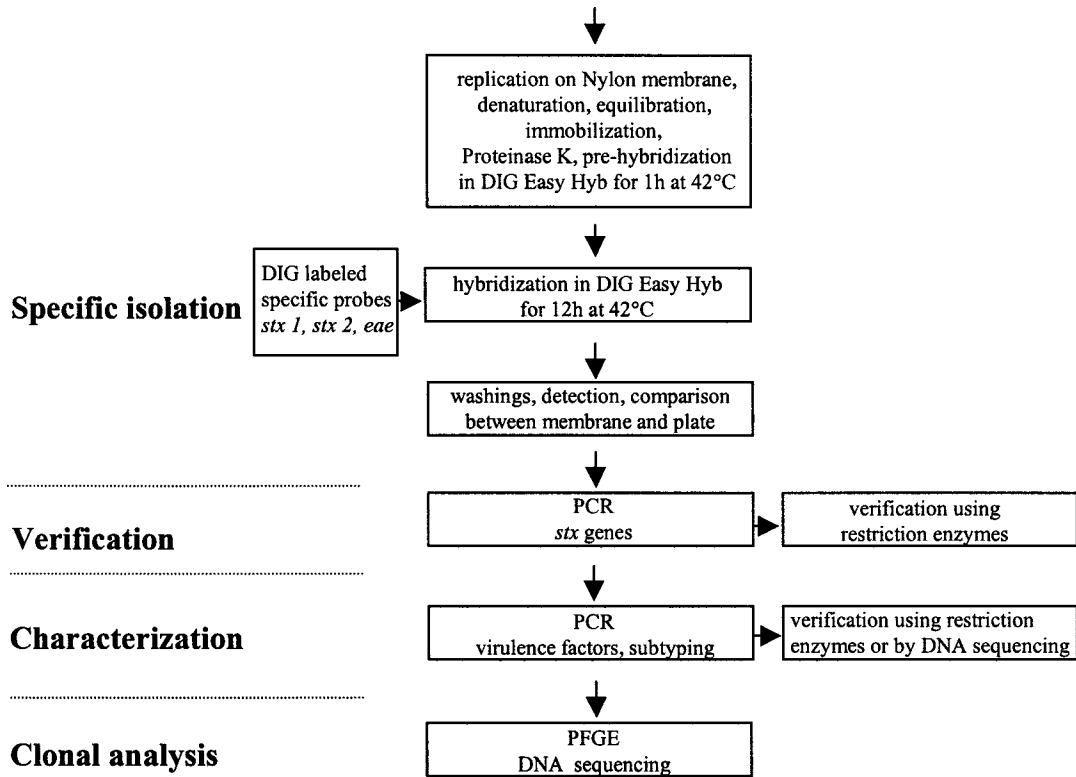
Fig. 2. Flow chart illustrating the general course of operation and the sequence of steps involved in the cascade of methods for specific detection, isolation, and characterization of STEC.
