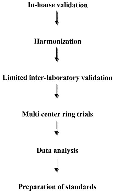
Fig. 5. The proper sequence of events in preparation of PCR standards.
